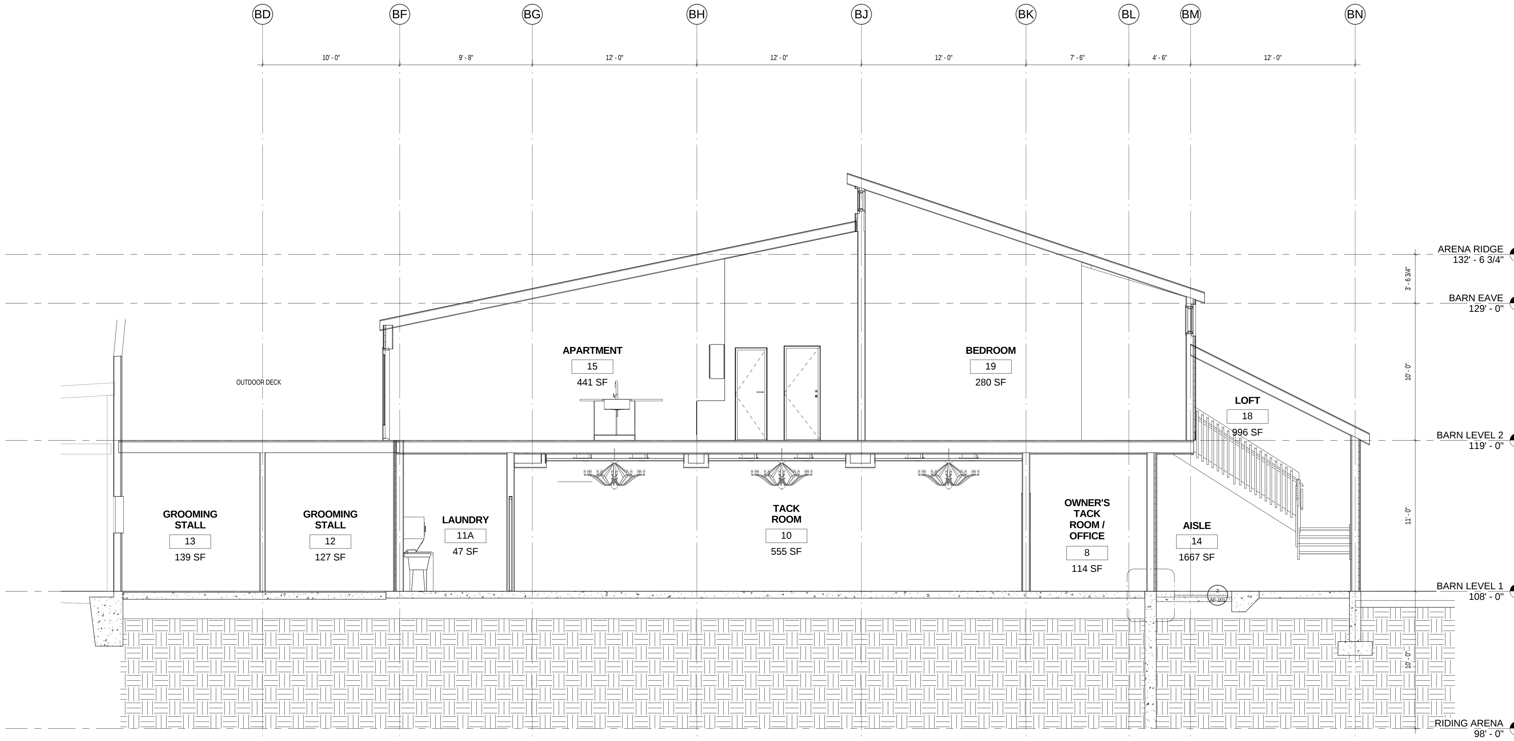
1 BUILDING SECTION 4 1/4" = 1'-0"
